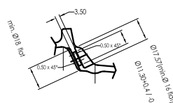
Section D Valve hole (Valve tool No. xxxxx)
